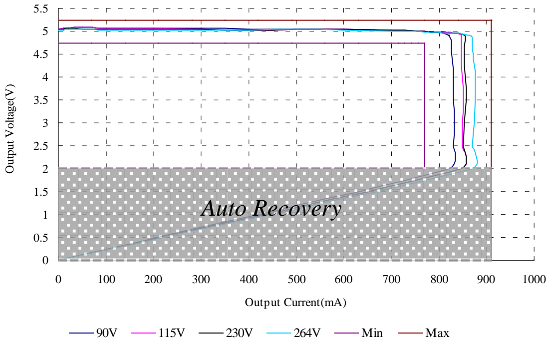
Fig. 3 I-V Curve
