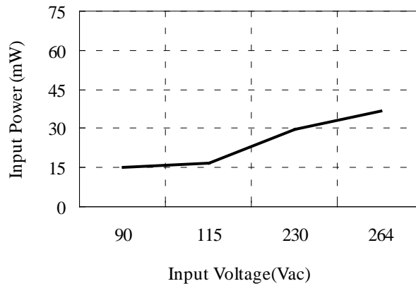
Fig. 1 Standby Power vs. Input Voltage
