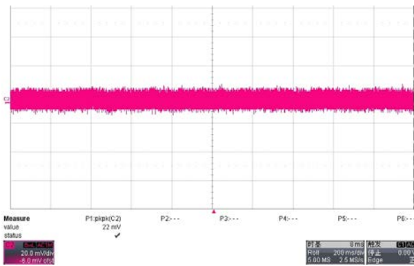
Fig. 6 Measured ripple& noise waveform@264V/50Hz, no load
