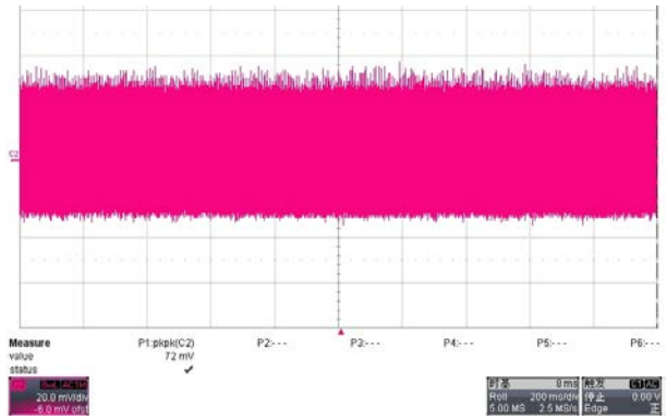
Fig. 5 Measured ripple& noise waveform@90V/60Hz, full load
