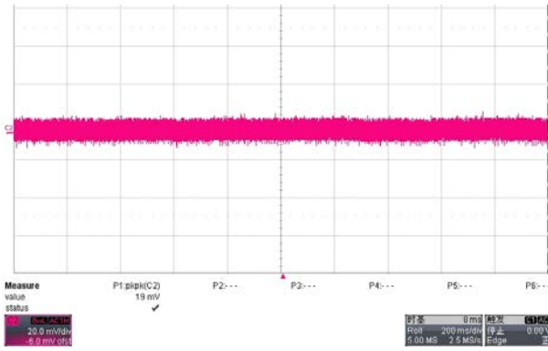
Fig. 4 Measured ripple& noise waveform@90V/60Hz, no load
