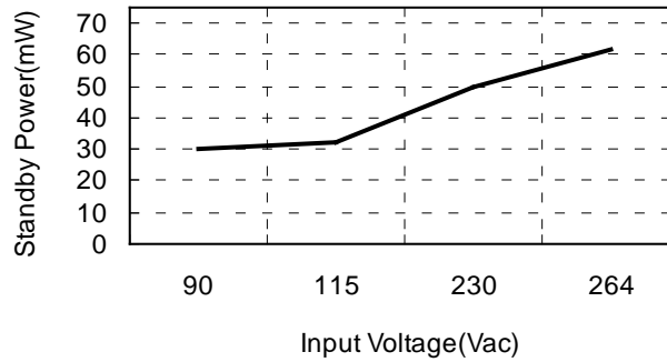
Fig. 1 Standby Power vs. Input Voltage
