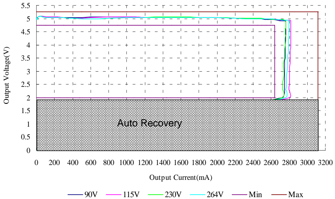
Fig. 3 I-V Curve
