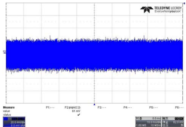
Fig. 7 Measured ripple&amp; noise waveform@264V/50Hz, full load
