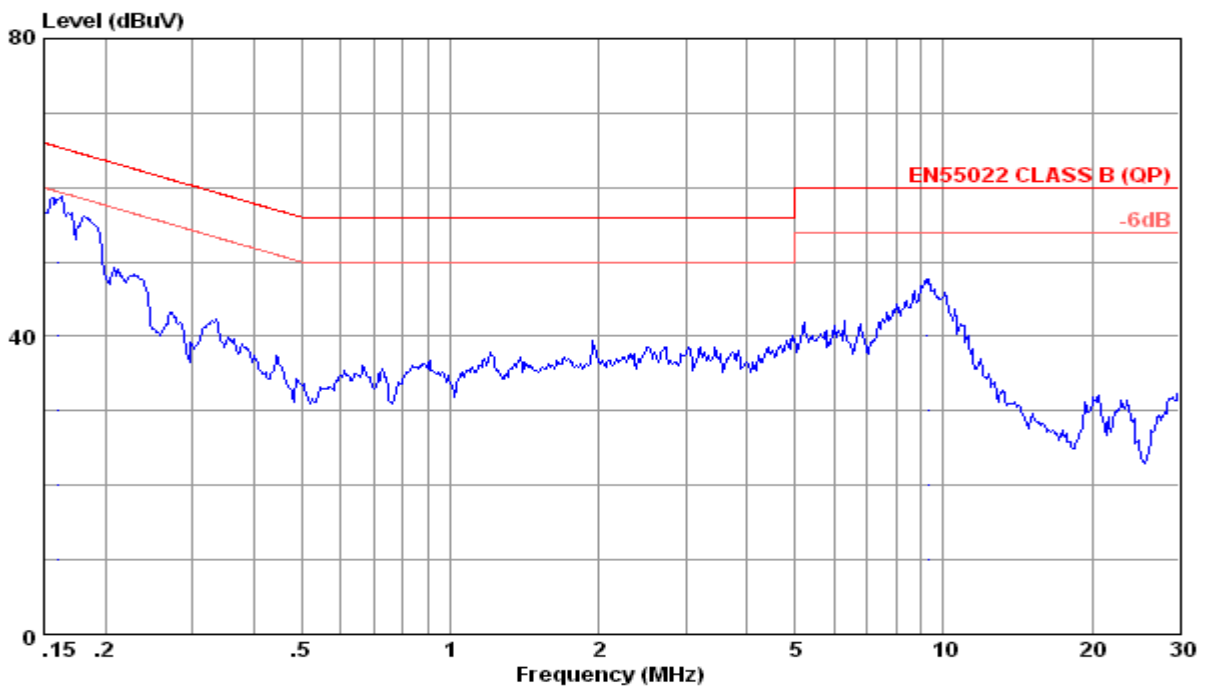
QP curve
